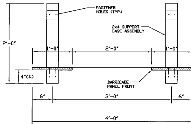
2 SUPPORT ASSEMBLY PLAN VIEW S-1 SCALE : 3/4" = 1'-0"
