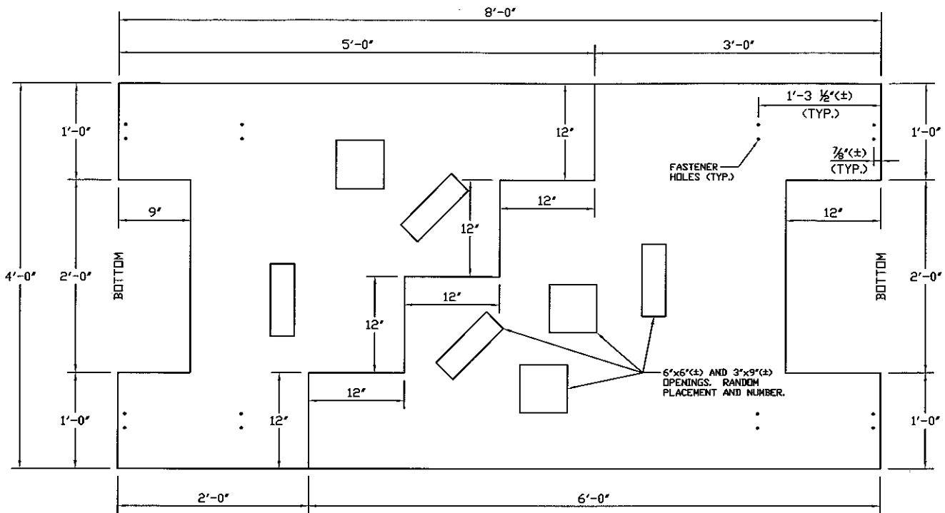
1 CUTTING LAYOUT S-1 SCALE : 3/4" = 1'-0"
